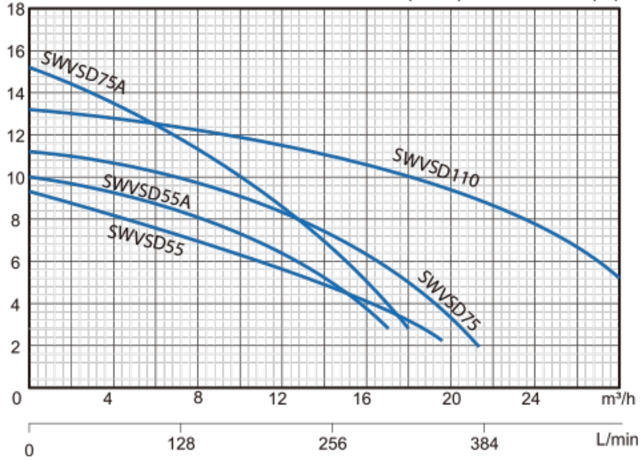
H (m) Performance chart at n=2850 r/min(50hz) Total head(m)
